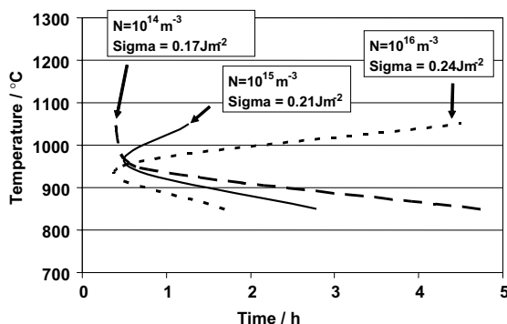
Fig. 4. Calculated time–temperature–precipitation diagram for VN particles in V1 steel.
