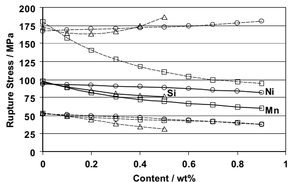
Fig. 2. Effects of nickel, silicon and manganese on the calculated creep rupture strength of steel V2 at 650 °C after 100 000 h. Solid lines represent the predictions and the error ranges are indicated by dashed lines with the same symbol.
