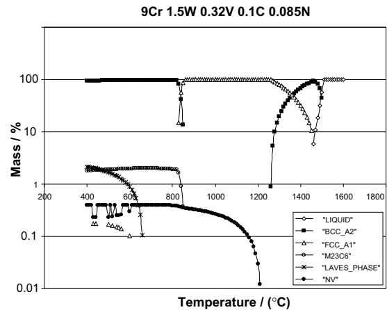
Fig. 1. Calculated equilibrium phase fractions for steel V1.
