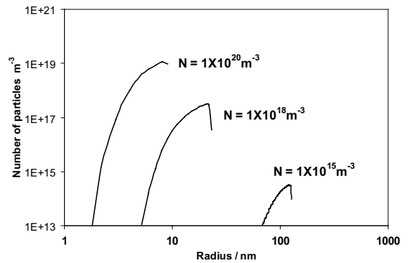
Fig. 5. Calculated size distribution at 950 °C of VN particles in V1 steel with various nucleation site densities. The interfacial energy used was 0.21 J m -2 .
