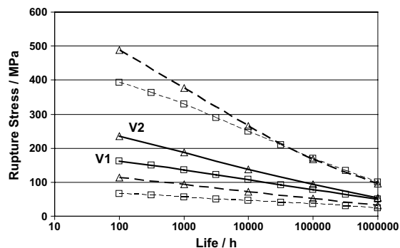
Fig. 3. Predicted creep rupture strength of alloys V1 and V2 at 650 °C. The solid and dashed lines have the same meaning as in Fig. 2.
